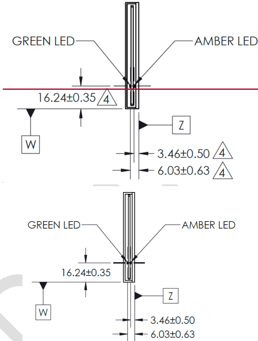
Figure 5-5. Front (LED Facing) Side of E2
