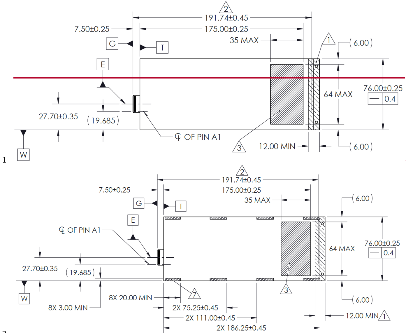
Figure 5-1. Primary Side of E2
