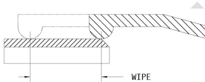
Figure 3-3 Wipe for a Continuous Contact
