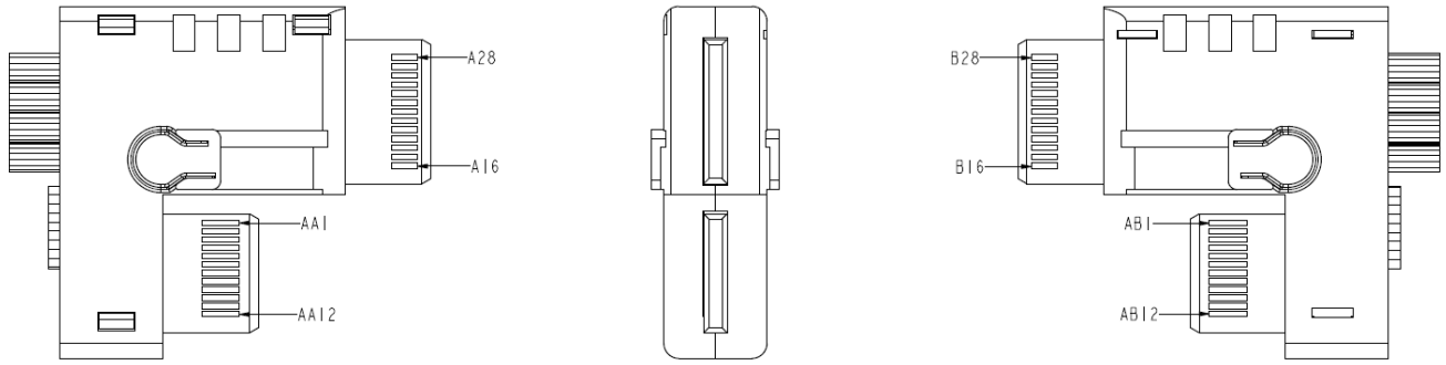
Figure 6-1 Contact Numbering for 1C-RS24 Connector Plug
