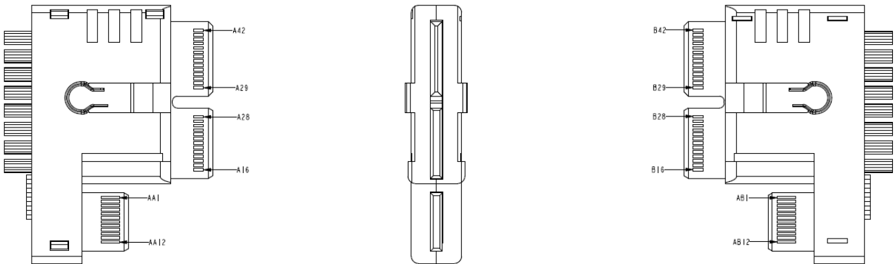
Figure 6-2 Contact Numbering for 2C-RS24 Connector Plug
