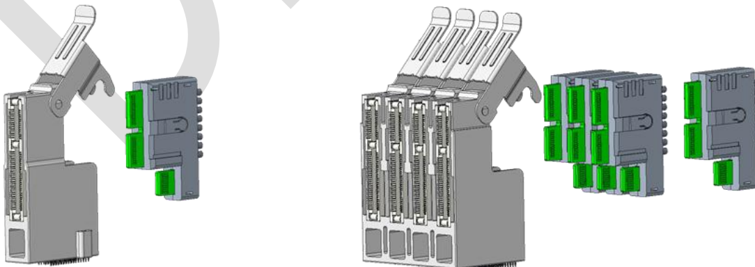
20 21 Figure 4-5 2C Hybrid Orthogonal Connector Receptacle and Plug with RS20 22
