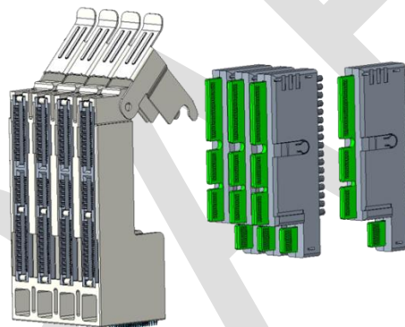
9 10 Figure 4-7 4C Hybrid Orthogonal Connector Receptacle and Plug with RS20
