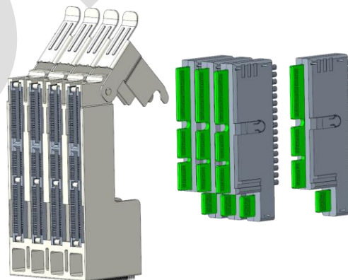
15 16 Figure 4-8 4C Hybrid Orthogonal Connector Receptacle and Plug with RS24
