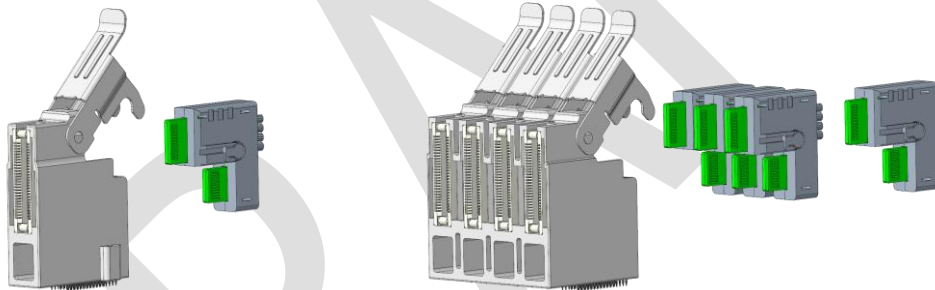
14 15 Figure 4-4 1C Hybrid Orthogonal Connector Receptacle and Plug with RS24
