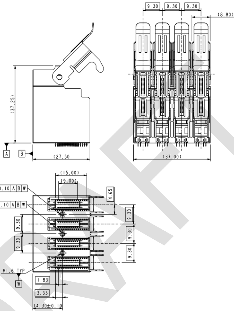
Figure 5-2 Ganged 1C-RS20 Connector
