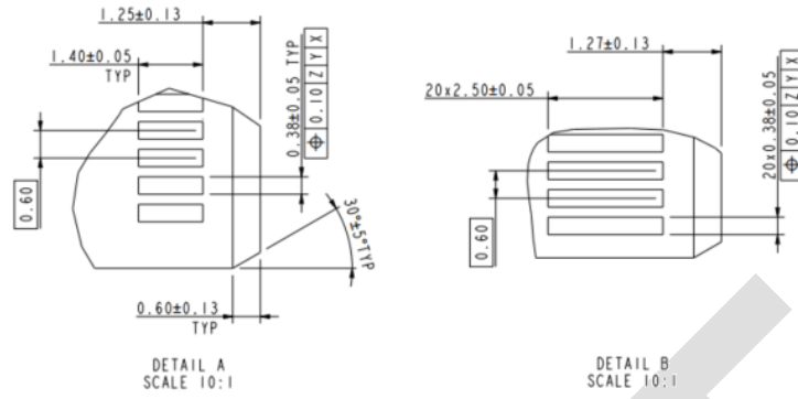
Figure 6-3 2C-RS20 Plug Module
