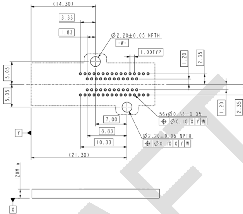
Figure A-2 Recommended Standalone Connector Footprint with RS24
