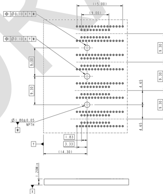
Figure A-3 Recommended Ganged Connector Footprint with RS20
