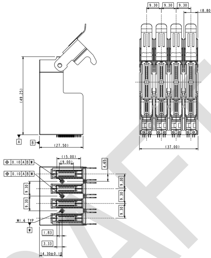
Figure 5-6 Ganged 2C-RS20 Connector
