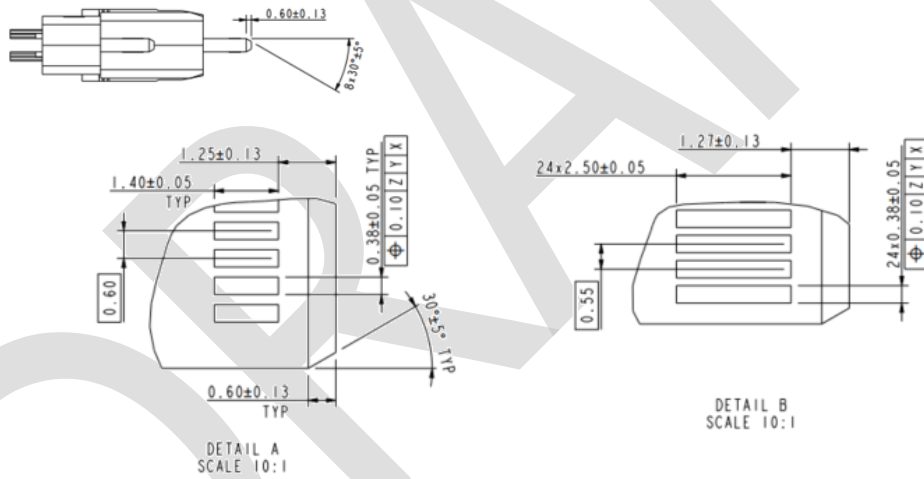
Figure 6-6 4C-RS24 Plug Module
