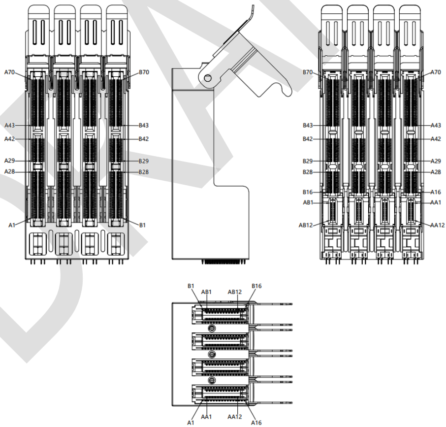
Figure 4-10 Contact Numbering of Receptacle Connectors with RS24
