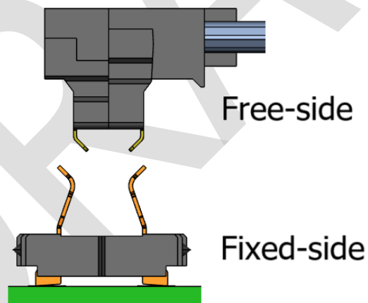
28 29 Figure 3-1 Fixed-side and Free-side Connector Definition
