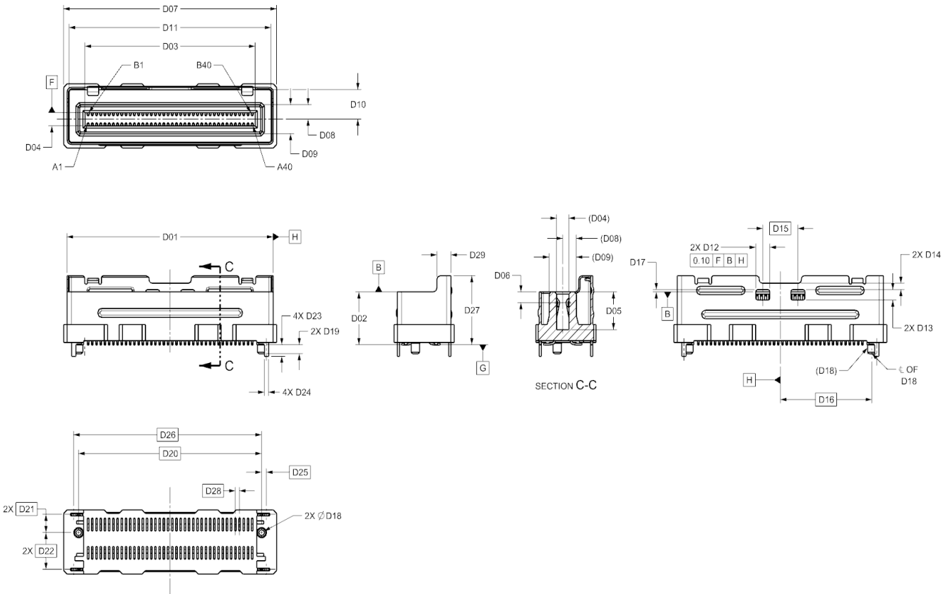
Figure 5-9 Vertical Connector with 80 Contacts
