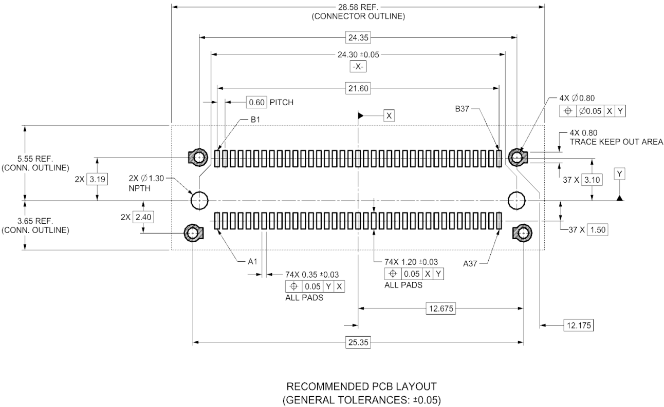
Figure 8-6 Recommended Footprint for Vertical 74P Connector Receptacle
