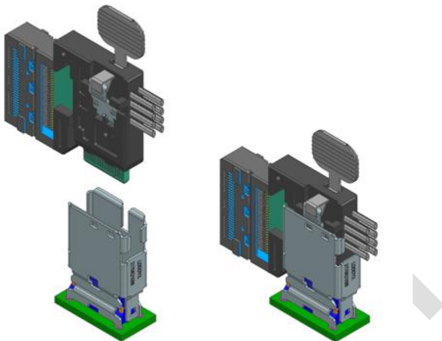
Figure 4-21 38-Pin Style B Connector Receptacle Unmated and Mated with E1-1C Plug
