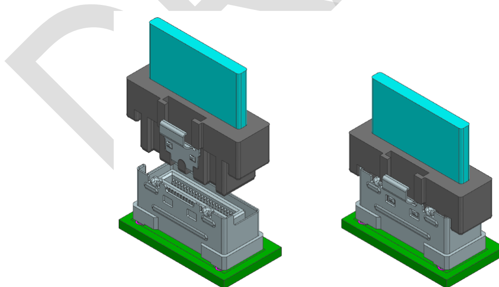
Figure 4-4 Configuration 3 – Unmated and Mated
