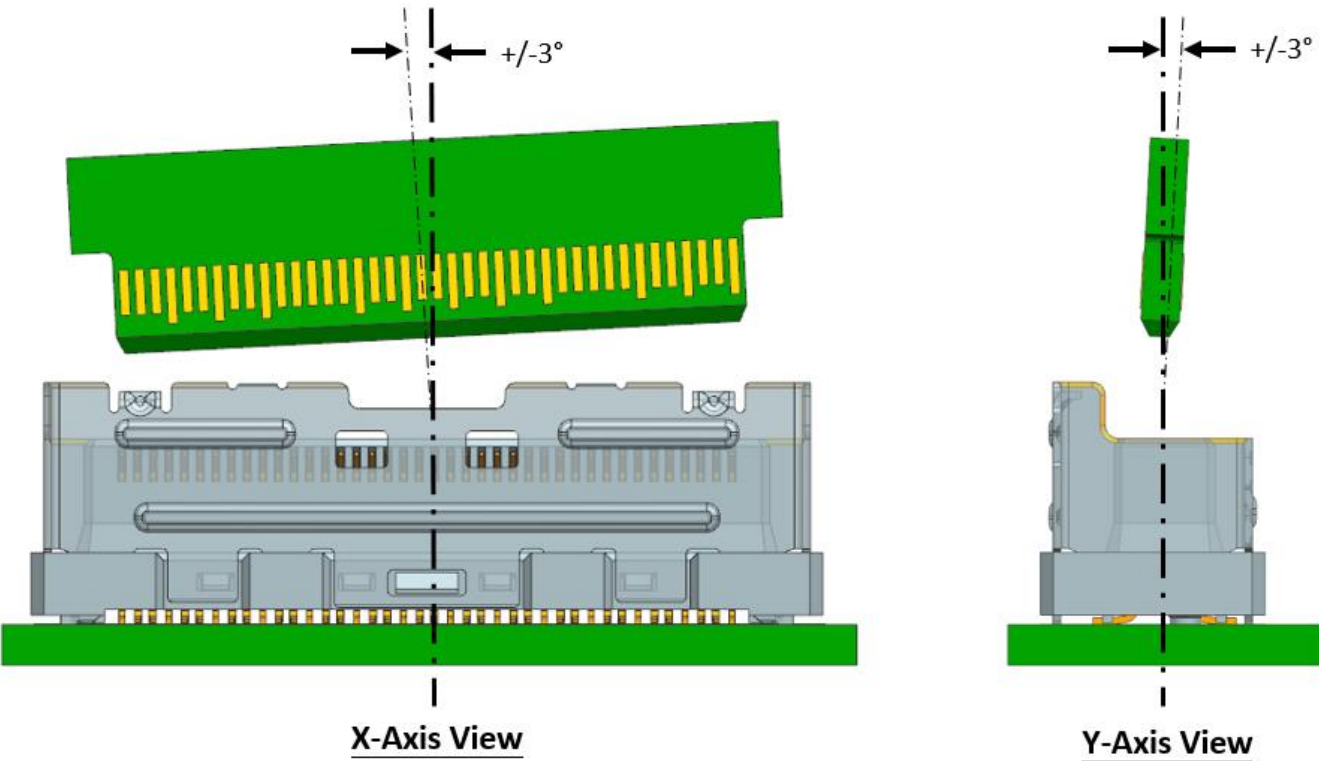
Figure 8-19 Angular Gatherability
