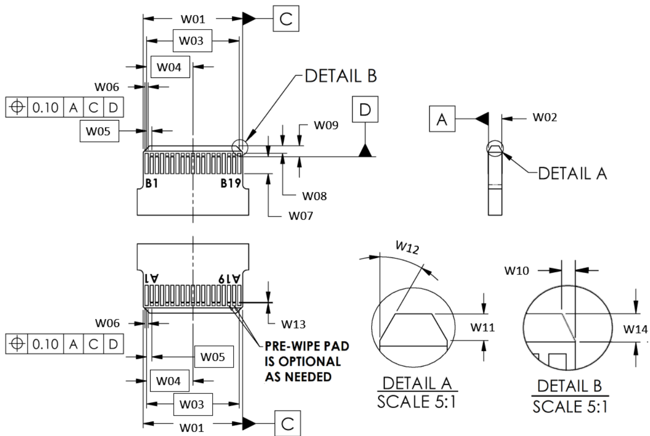
Figure 6-14 Paddle-Card Description for 38-Pin Style A & B Connector Receptacles
