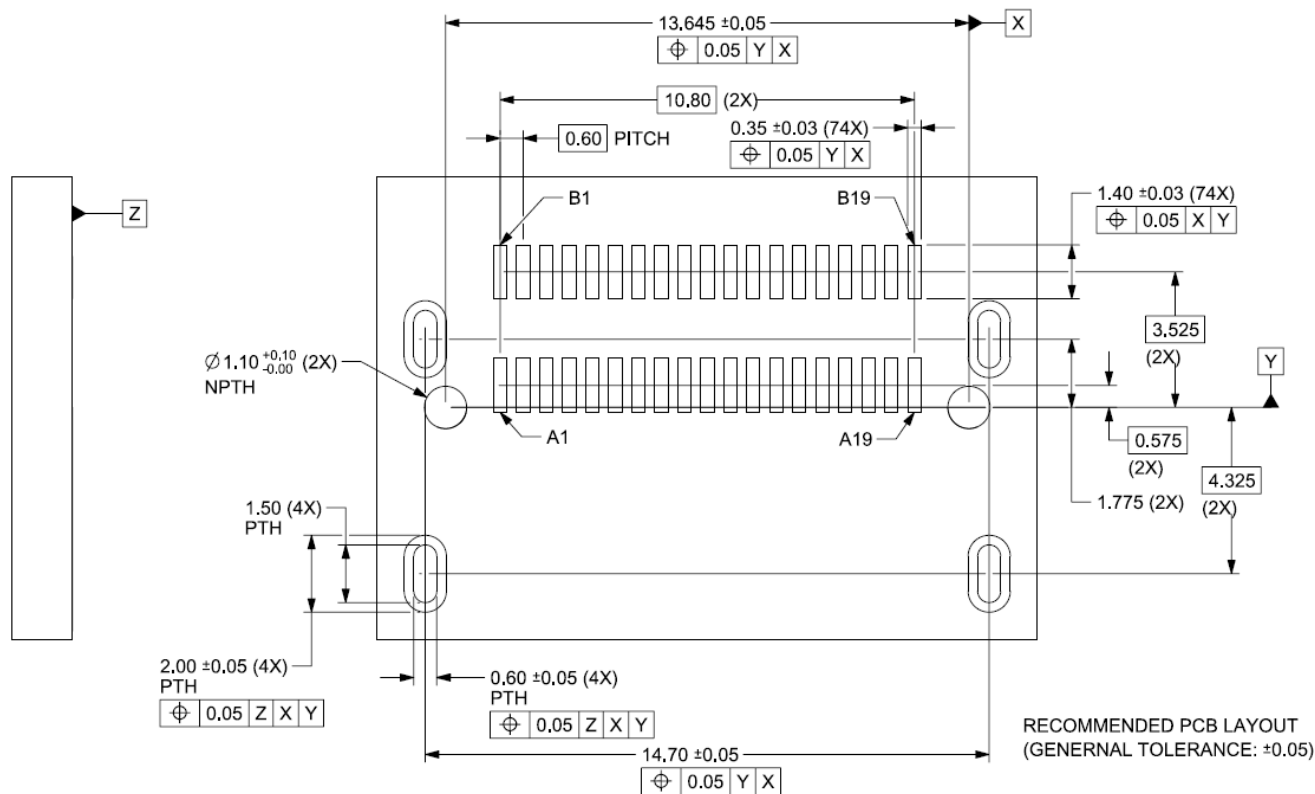
Figure 8-2 Recommended Footprint for Right Angle 38P Style A Connector Receptacle
