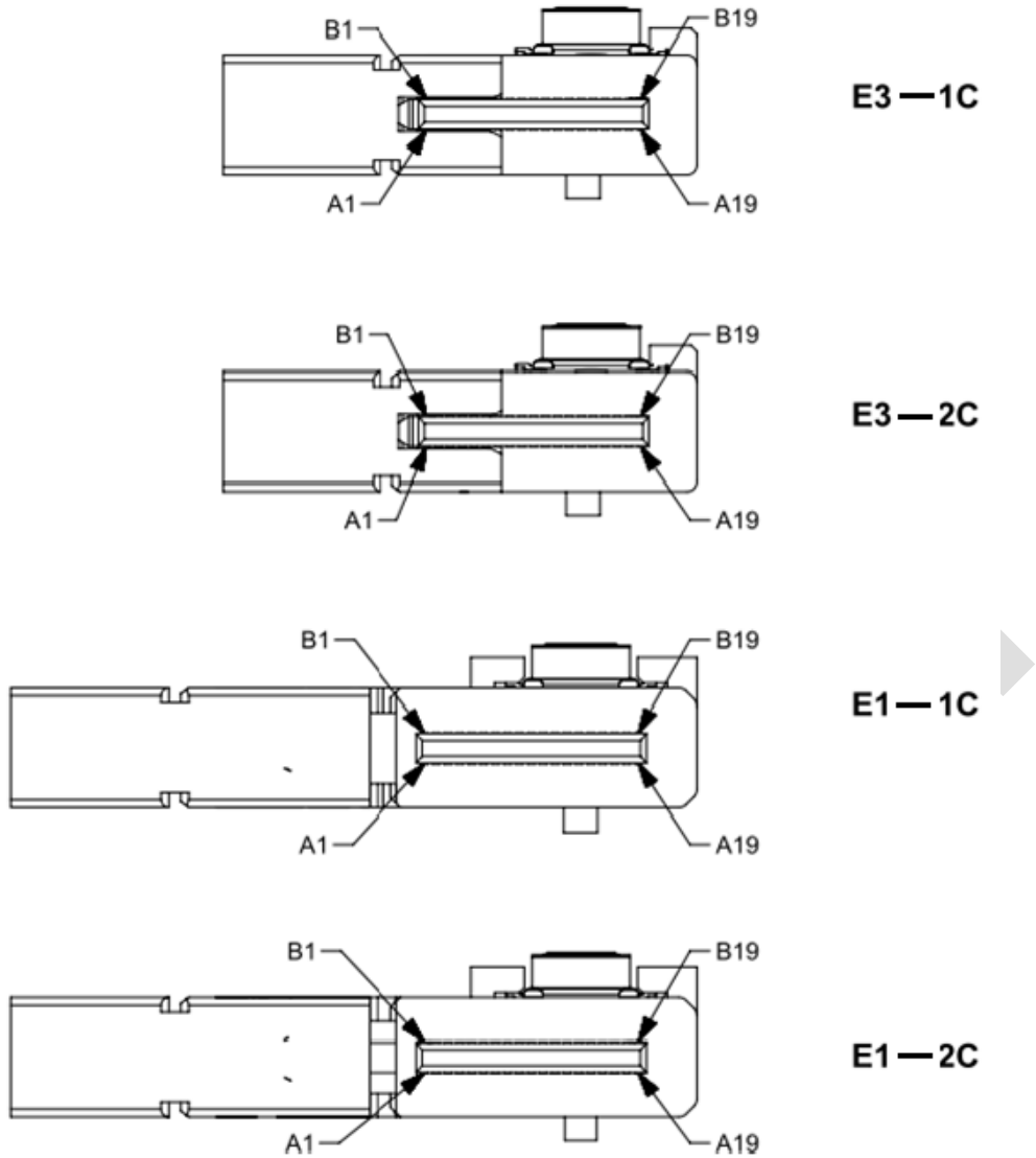
Figure 4-24 Contact Numbering for 38-Pin Style B Connector Plug
