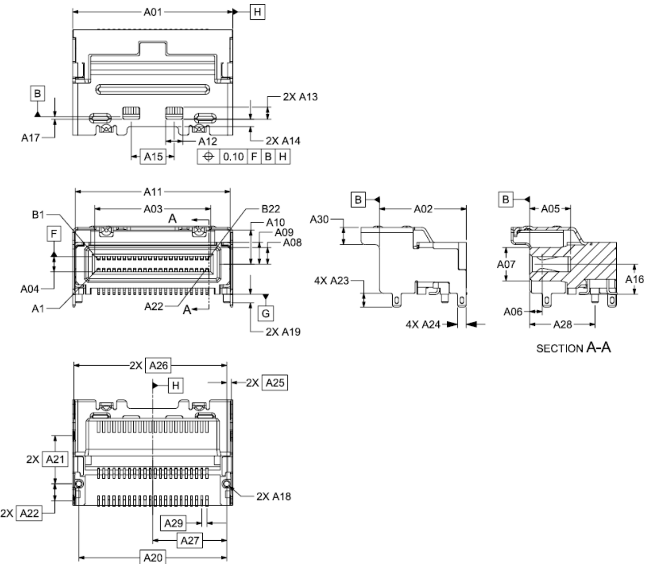
Figure 5-15 Right-Angle Connector with 44 Contacts
