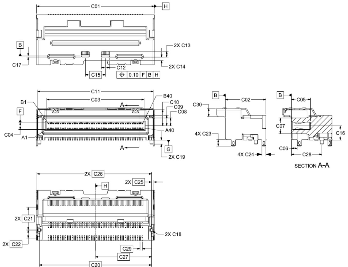
Figure 5-17 Right-Angle Connector with 80 Contacts
