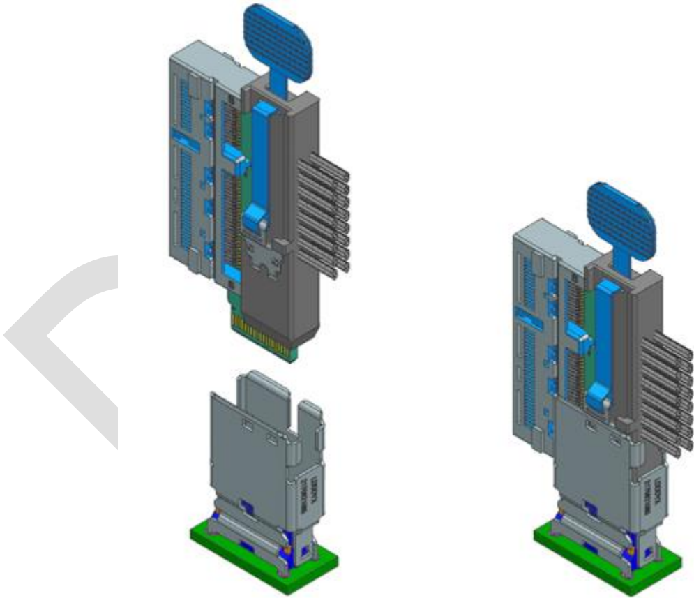
Figure 4-18 38-Pin Style B Connector Receptacle Unmated and Mated with E3-2C Plug
