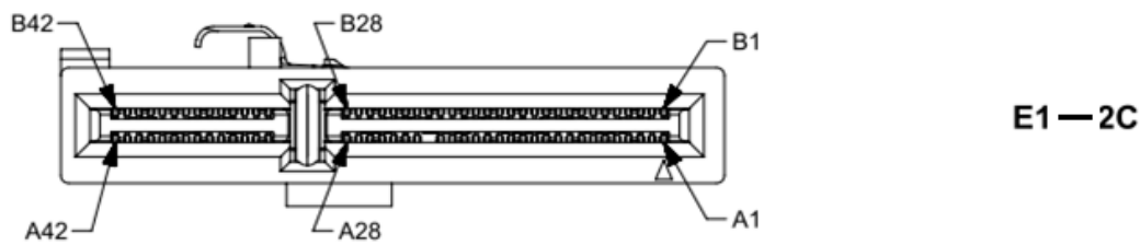
Figure 4-23 Contact Numbering for Gen-Z Connector
