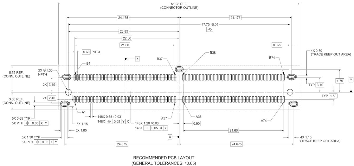
Figure 8-14 Recommended Footprint for Vertical 148P Connector Receptacle
