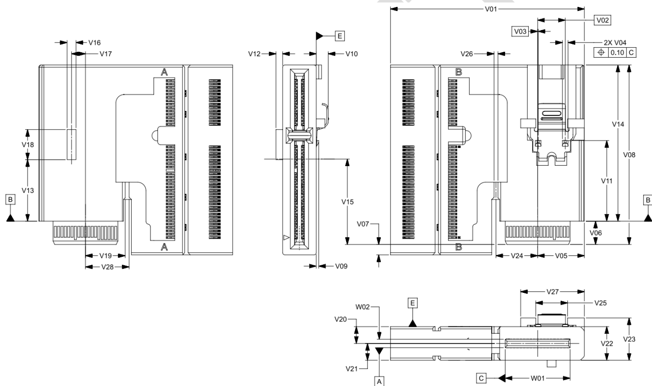
Figure 6-12 Dimensions of 38-Pin Style B Connector Plug E1-2C
