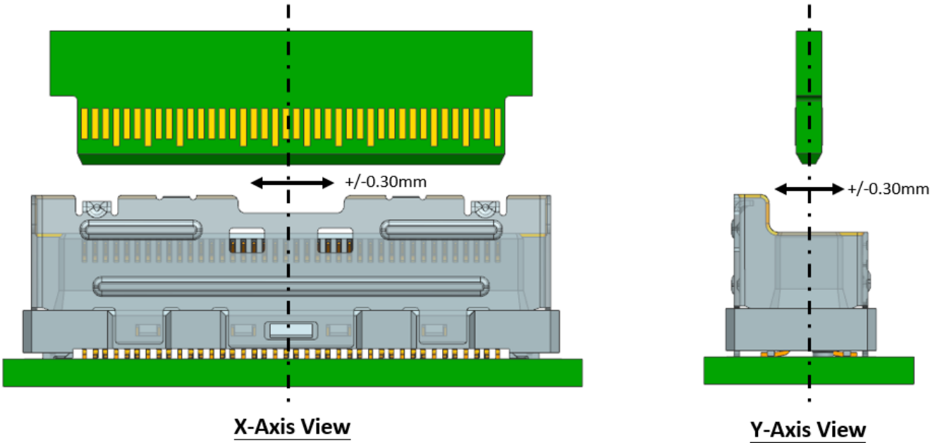
Figure 8-18 Linear Gatherability
