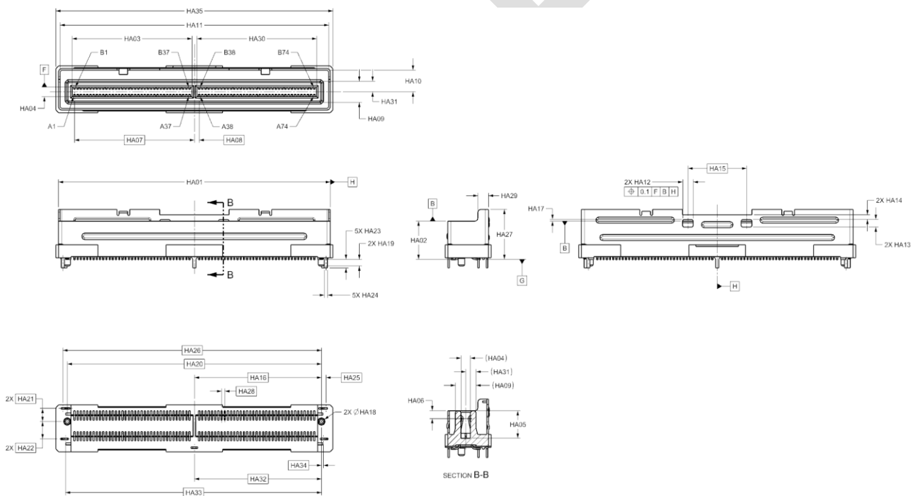
Figure 5-12 Vertical Connector with 148 Contacts
