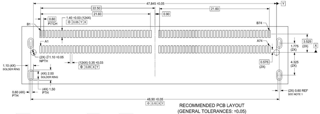
Figure 8-15 Recommended Footprint for Right Angle 148P Connector Receptacle
