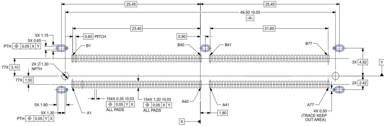
RECOMMENDED PCB LAYOUT (GENERAL TOLERANCES: ±0.05)
