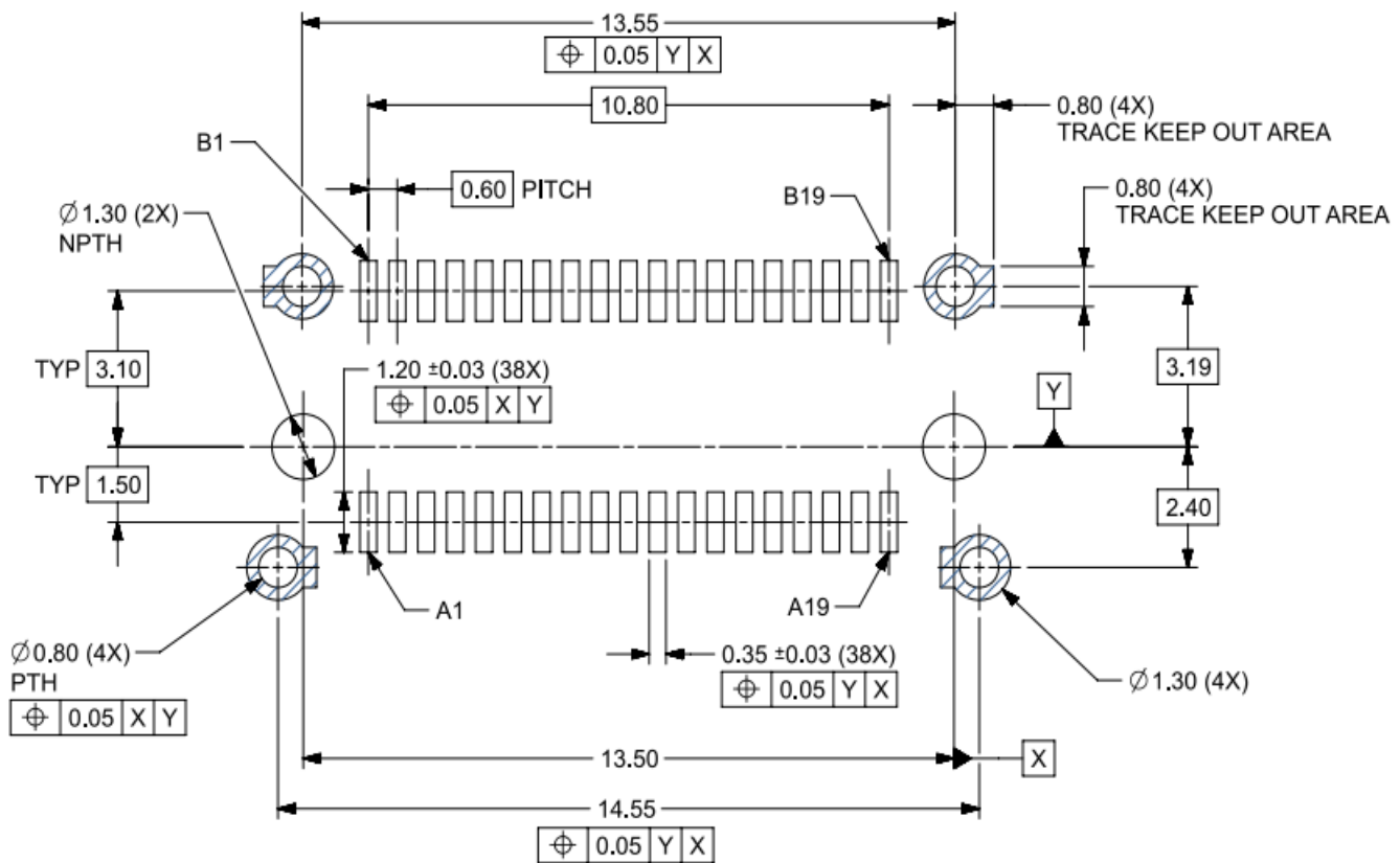
RECOMMENDED PCB LAYOUT (GENERAL TOLERANCE: +/-0.05) Figure 8-1 Recommended Footprint for Vertical 38P Style A Connector Receptacle
