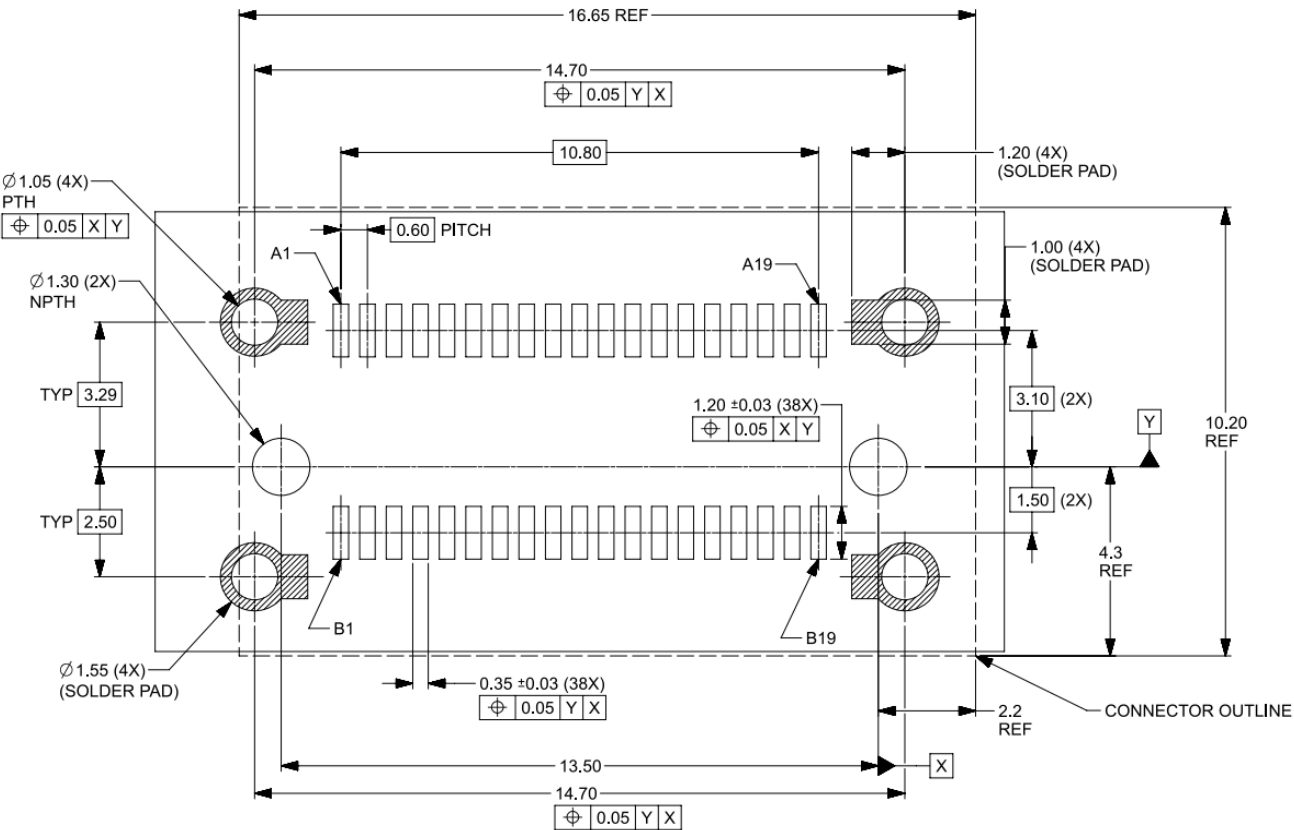
Figure 8-3 Recommended Footprint for Vertical 38P Style B "Ortho" Connector Receptacle
