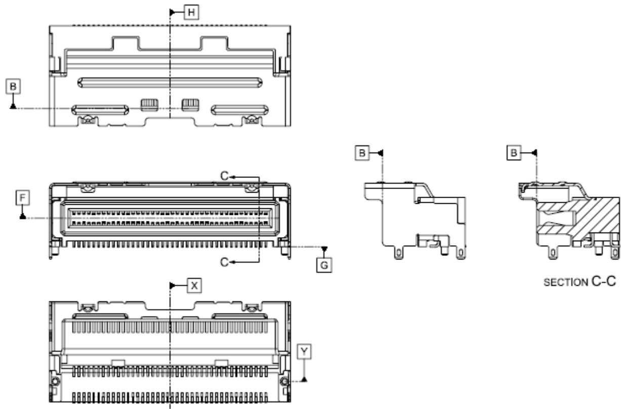
Figure 5-2 Right Angle Receptacle Datum Definitions
