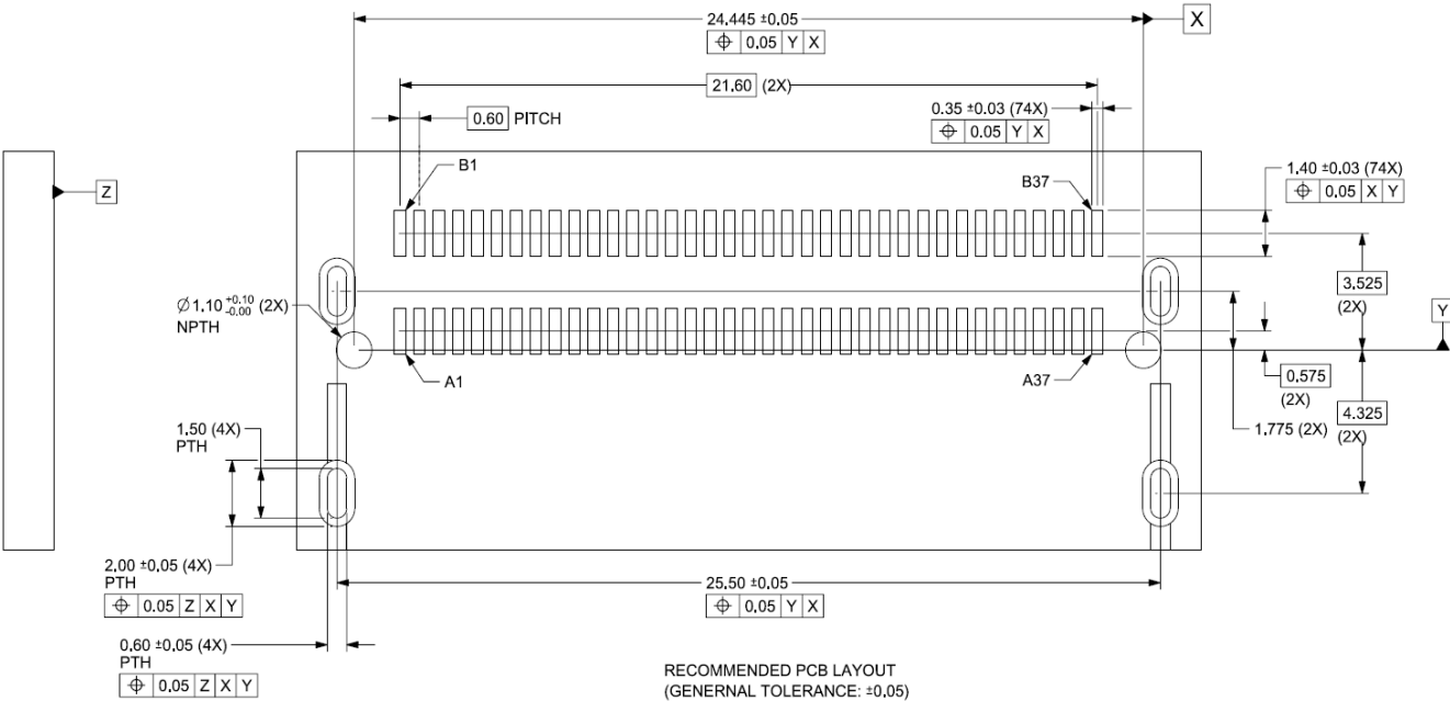
Figure 8-7 Recommended Footprint for Right Angle 74P Connector Receptacle
