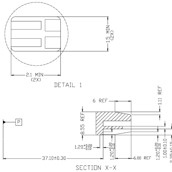
Figure 7-2 SFP2 High Speed Pads Viewing Windows
