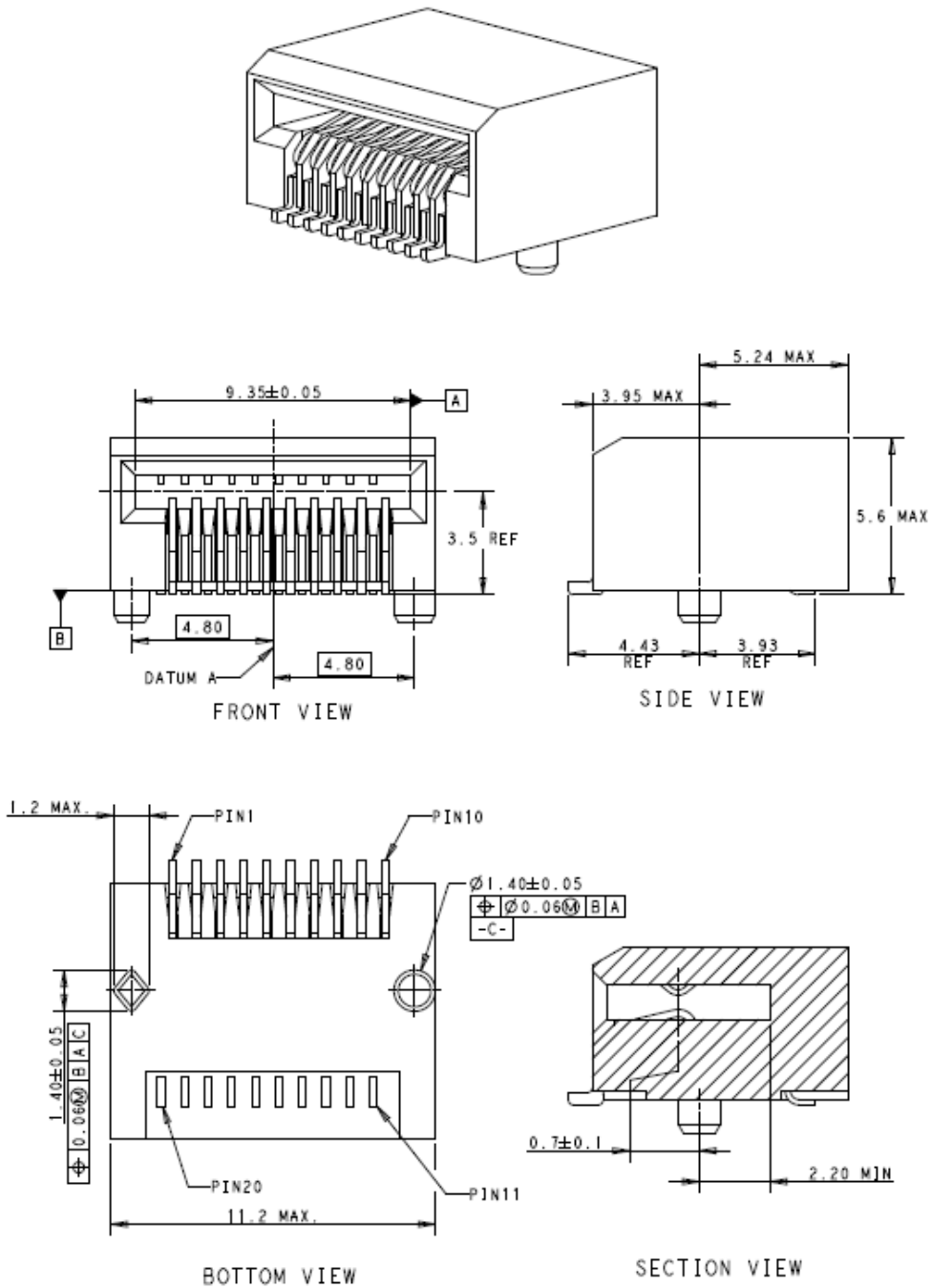
Figure 5-2 SFP2 SMT Connector
