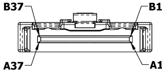
74 CONTACT PLUGS
