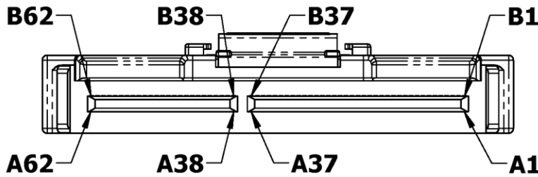
124 CONTACT PLUGS
