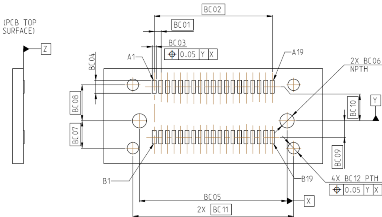
Figure A-5 Recommended Footprint for Hybrid Standard Vertical 38P Connectors
