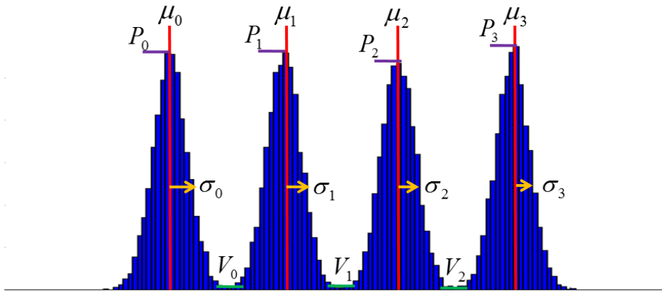
Figure 6-2 PAM4 vertical slice histogram
