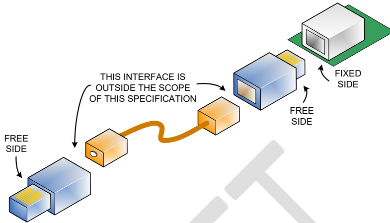
Figure 4-3 Separable Transceiver Module Implementation
