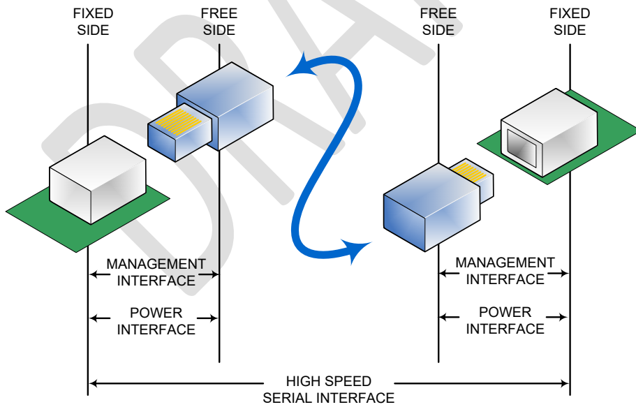
Figure 4-4 Management Interface Scope
