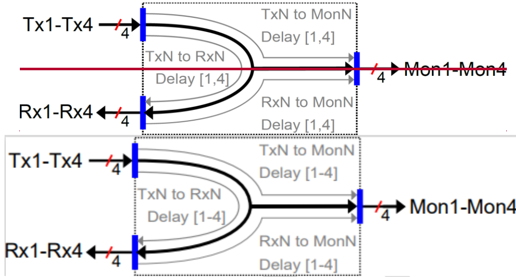
Figure 7-1 Calibration Loopback Module
