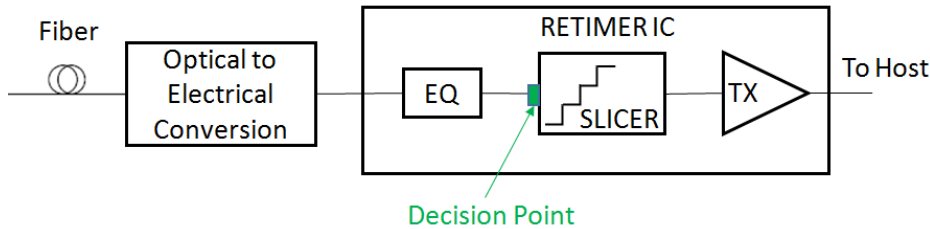
Figure 6-1 Optical ingress path of Module
