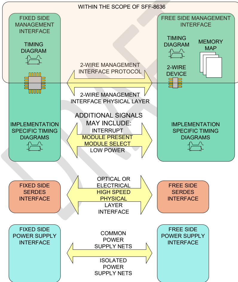
Figure 4-1 Common Management Interface Block Diagram
