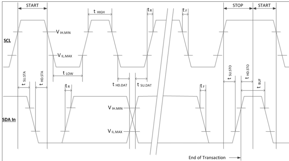
Figure 5-7 Timing Diagram
