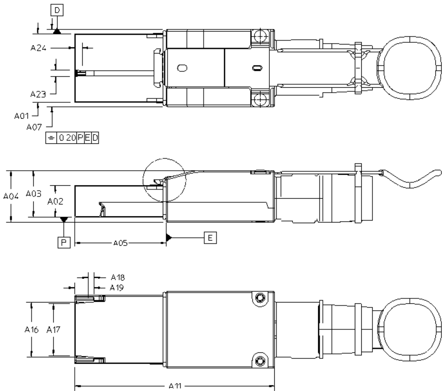
FIGURE 5-3 PLUG (2)
