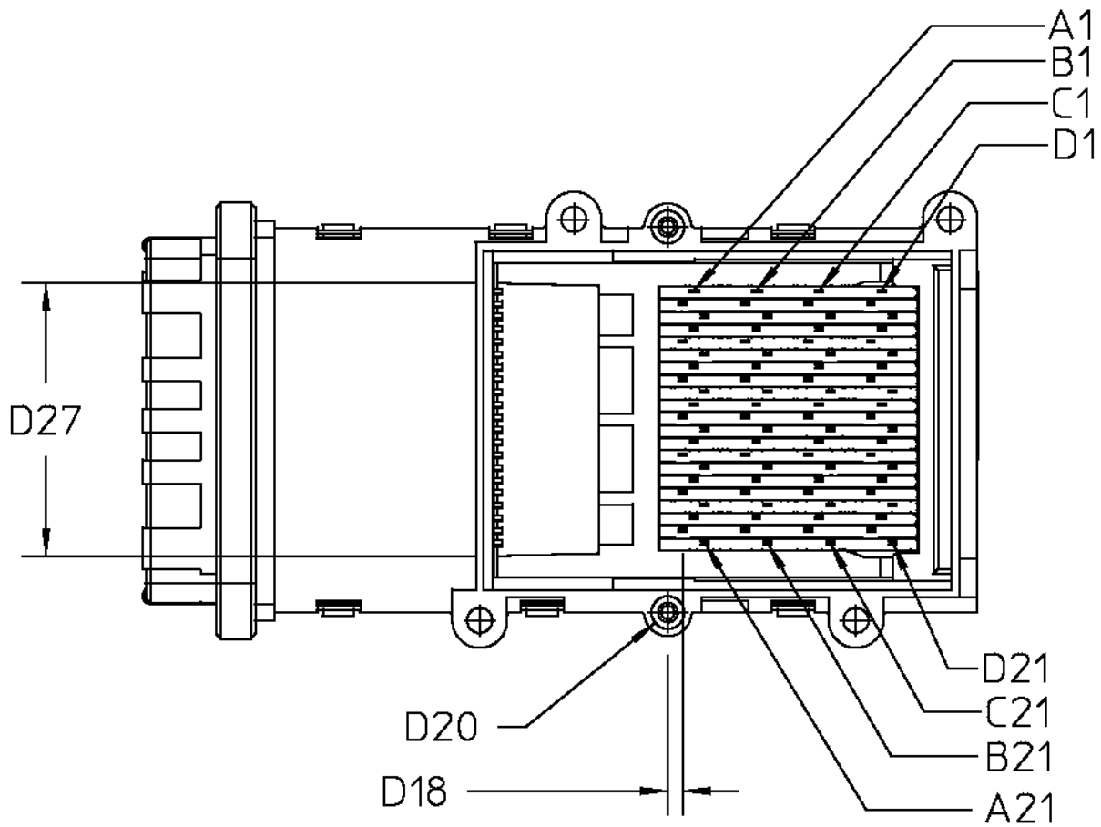
FIGURE 5-9 RECEPTACLE (3)
