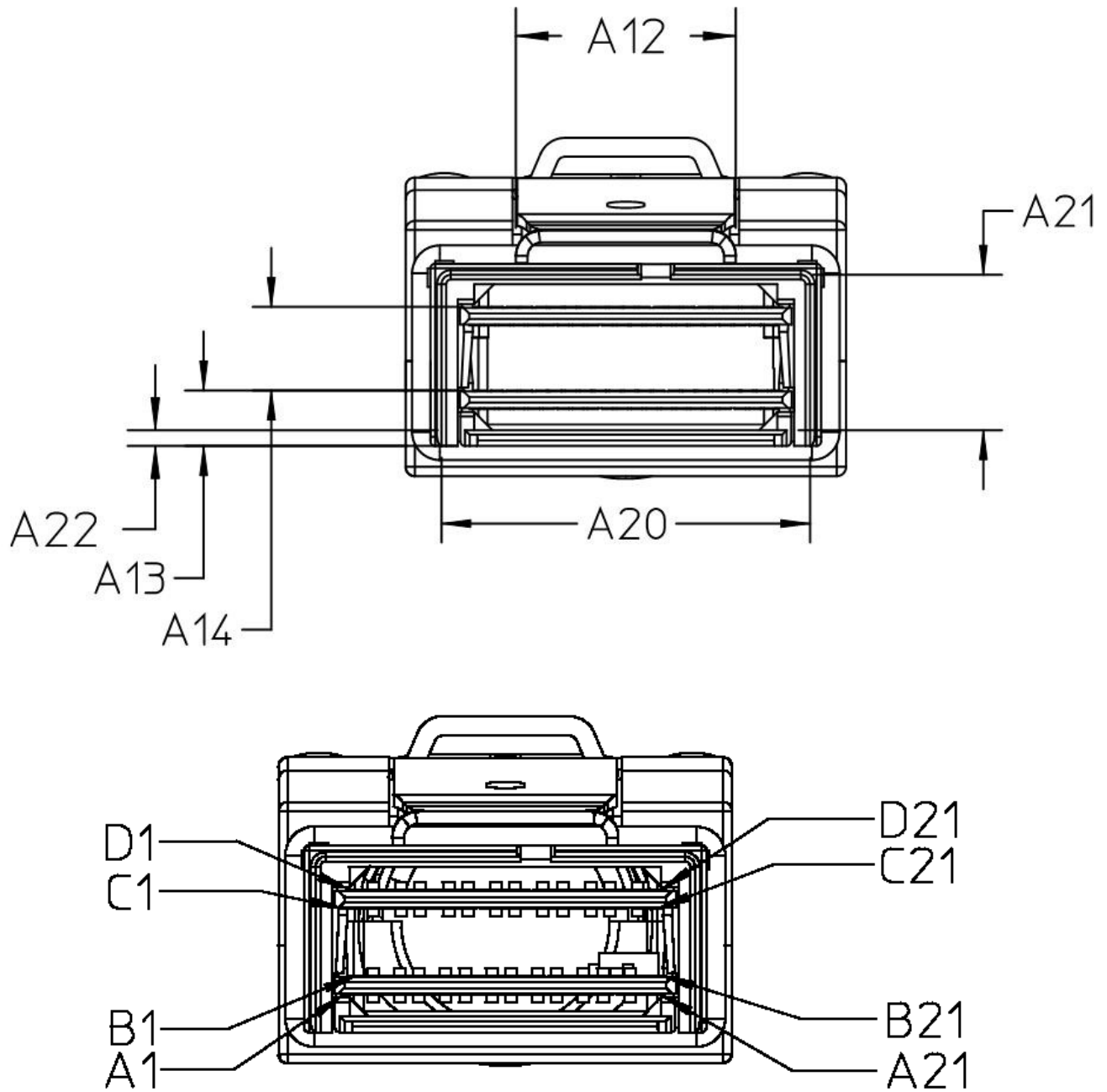
FIGURE 5-4 PLUG (3)
