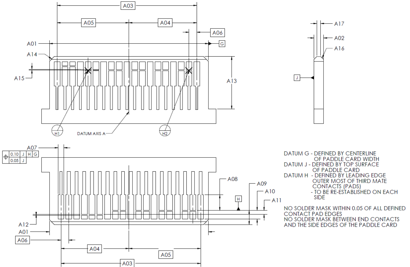
FIGURE 5-1 FREE (MODULE) PADDLE CARD
