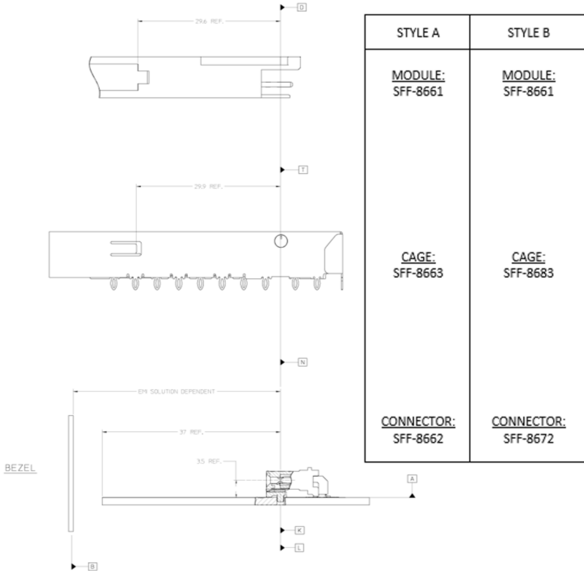
FIGURE 4-1 DATUM DEFINITIONS
