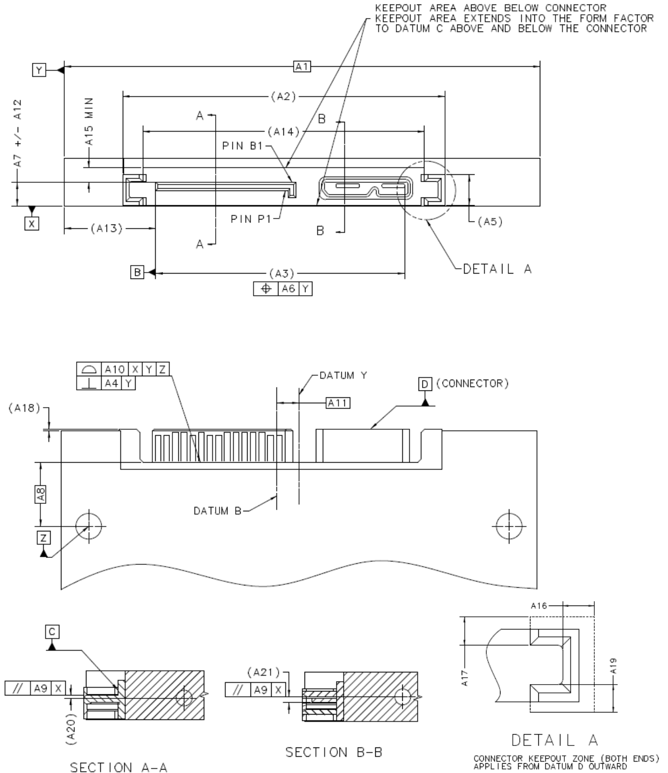
FIGURE 3-1 OPTION 1: 2.5" DRIVE FORM FACTOR WITH THE COMBINATION CONNECTOR INCLUDING A USB 3.0 MICRO-B RECEPTACLE REFERENCED TO BOTTOM MOUNTING SCREWS
