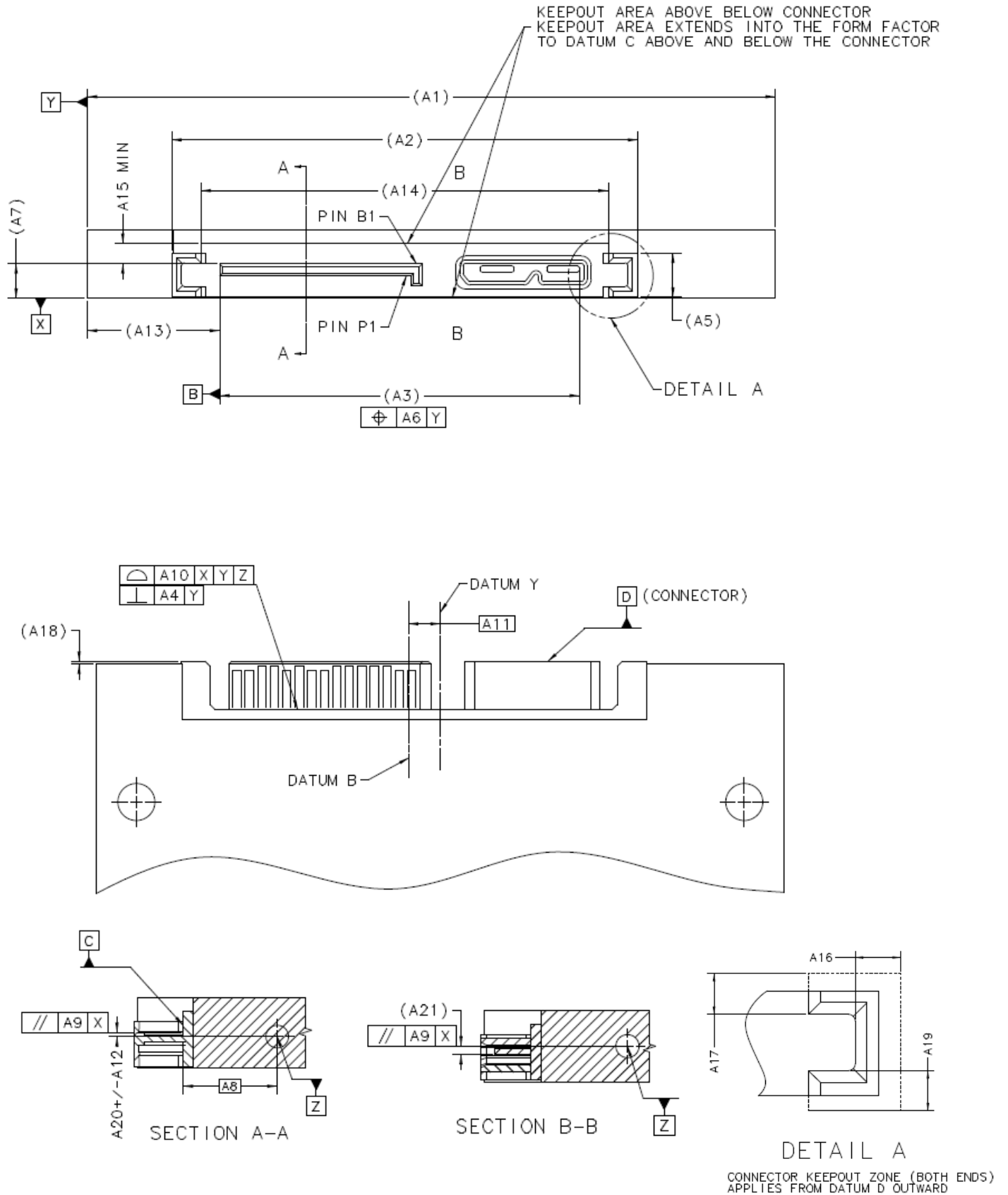
FIGURE 3-2 OPTION 2: 2.5" DRIVE FORM FACTOR WITH THE COMBINATION CONNECTOR INCLUDING A USB 3.0 MICRO-B RECEPTACLE REFERENCED TO SIDE MOUNTING SCREWS
