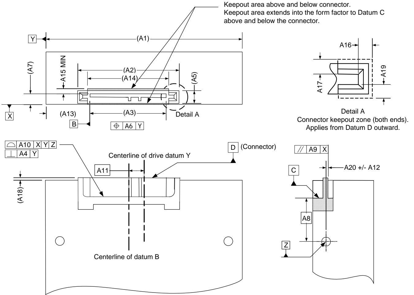
FIGURE 3-2 OPTION 2: 2.5" DRIVE FORM FACTOR WITH SERIAL CONNECTOR REFERENCED TO SIDE MOUNTING SCREW
