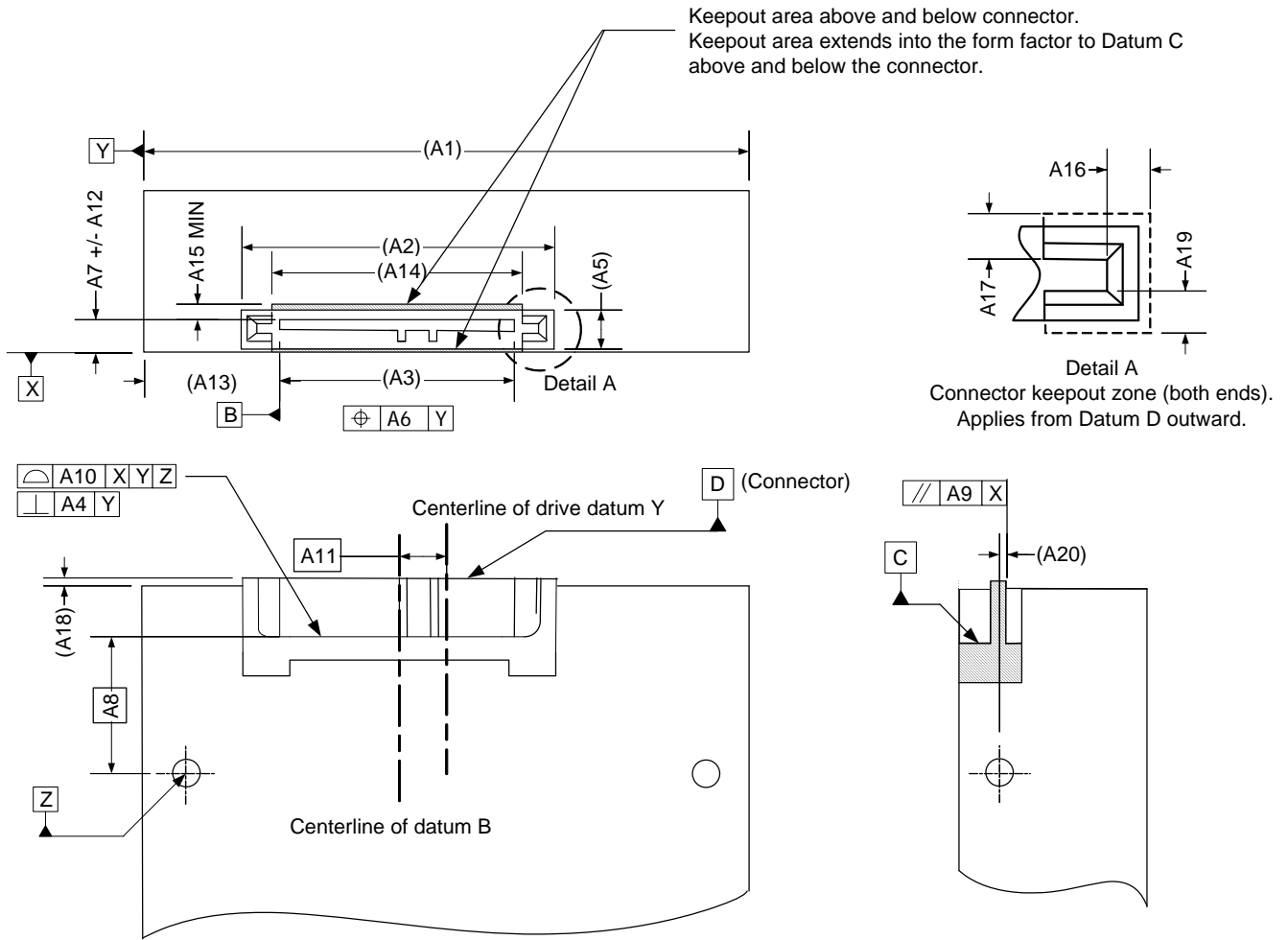
FIGURE 3-1 OPTION 1: 2.5" DRIVE FORM FACTOR WITH SERIAL CONNECTOR REFERENCED TO BOTTOM MOUNTING SCREW
