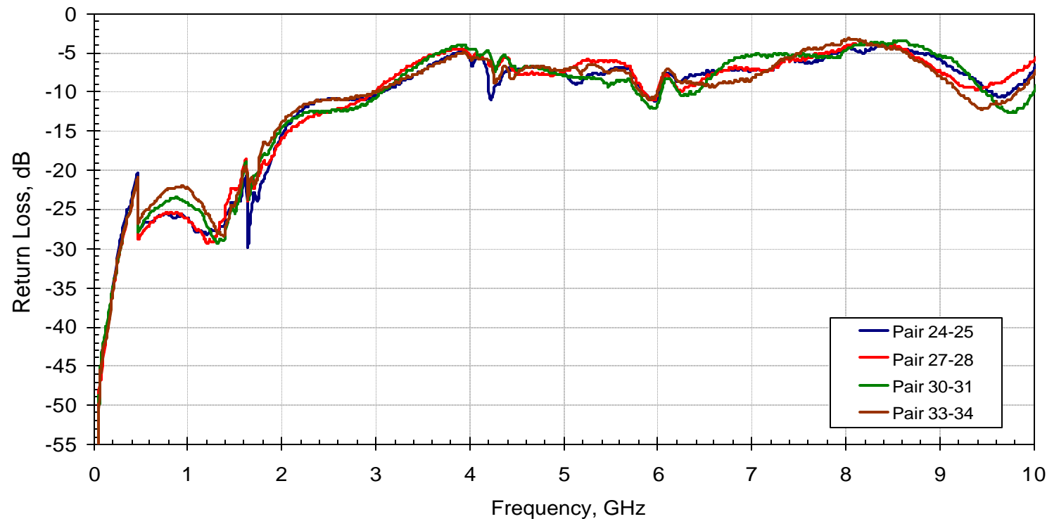
Return Loss Extended Vertical Receptacle to Straddle Mount Plug
